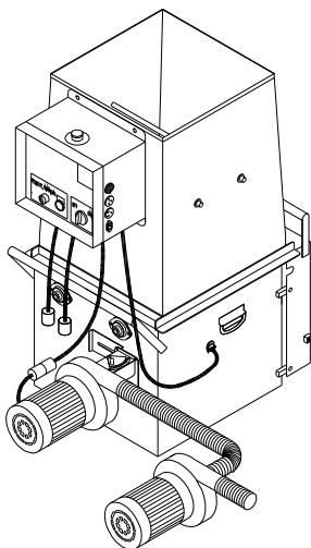
IN-LINE BLOWER SYSTEM
