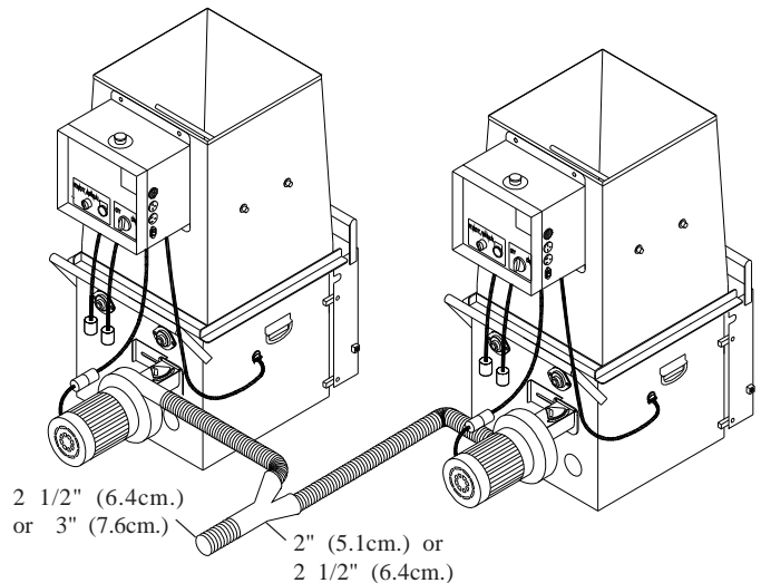
PARALLEL BLOWER SYSTEM
